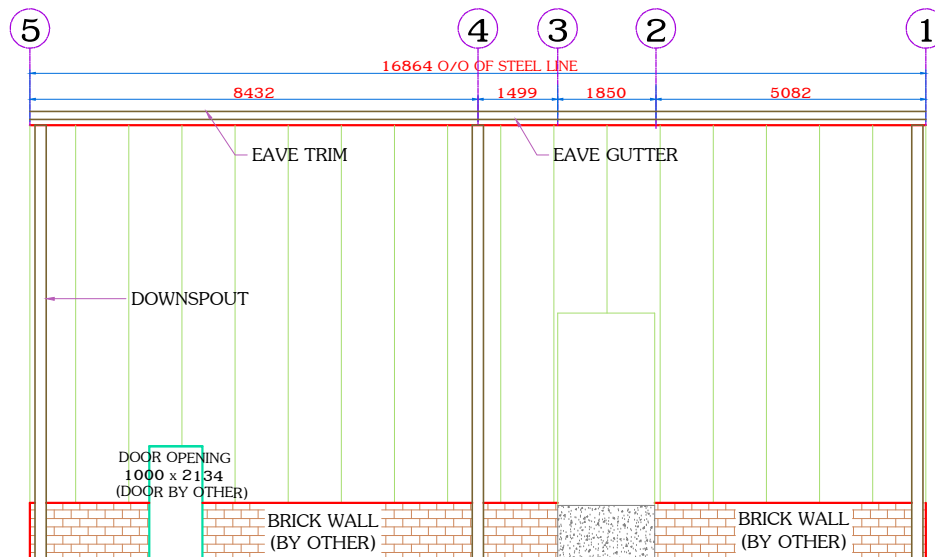
SIDE WALL SHEETING @ GRID-A
