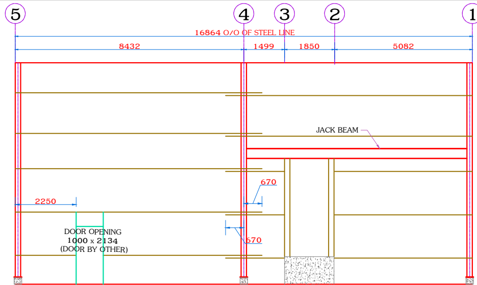
SIDE WALL FRAMING @ GRID-A
